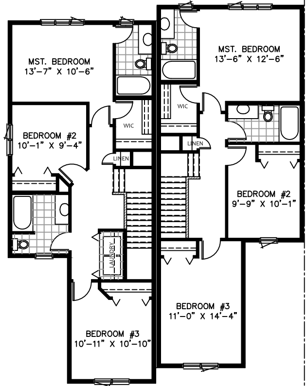
SECOND FLOOR B1 778 Sq. Ft.
