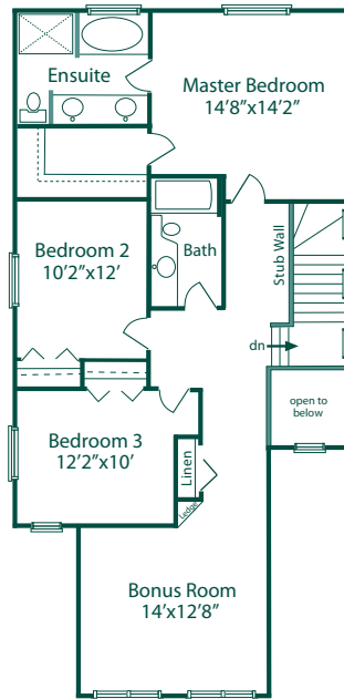
Upper Level 1,099 Sq. Ft.
