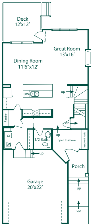
Main Level 904 Sq. Ft.
